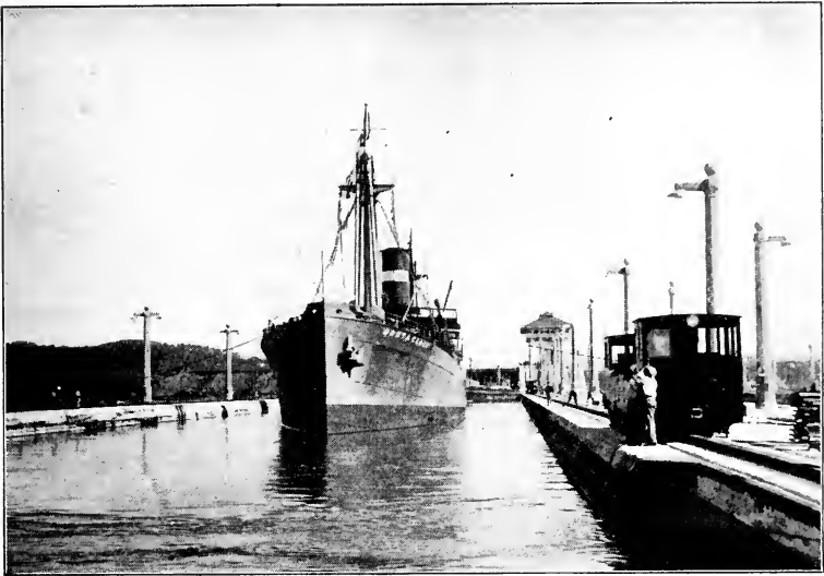
PANAMA CANAL: at the Ninaflores Locks, looking north, showing S. S. Santa Clara in lower west chamber, ready for water to be lowered to sea level.
